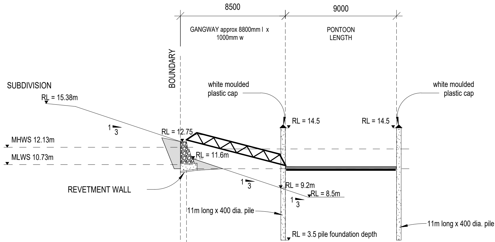
TYPICAL SECTION - JETTY TYPE END ON
